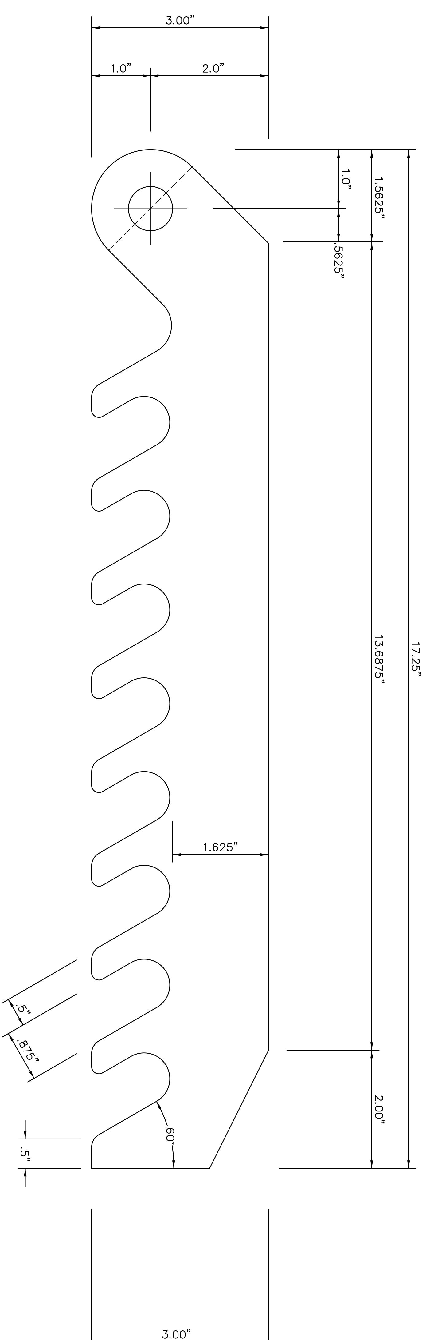
RATCHET ARM 3"x1/2" C.R. STEEL 1 EACH REQUIRED
