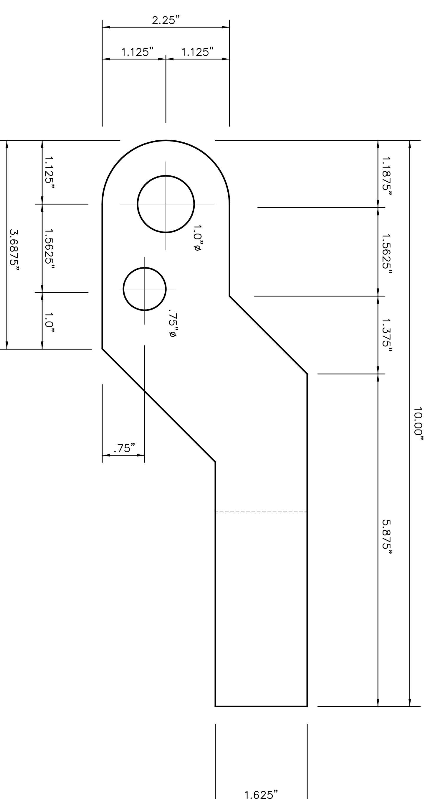
CONTROL LEVER TOP VIEW
