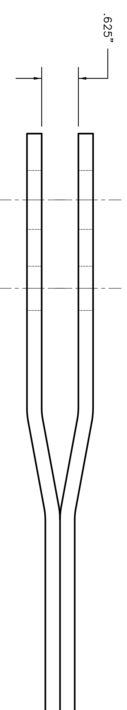
CONTROL LEVER SIDE VIEW 1/4" C.R. STEEL 2 OF EACH REQUIRED
